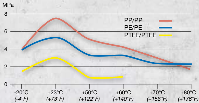
Tensile shear strength of WEICON Easy-Mix PE-PP 45 compliant with DIN EN 1465 in temperature curve
