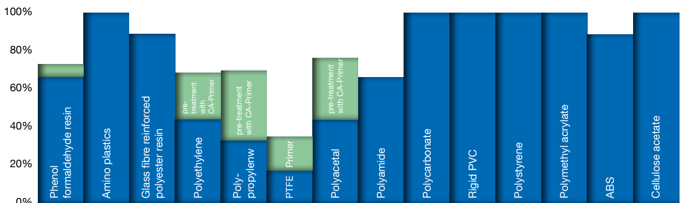
Combined tension and shear resistance (DIN EN 1465) / ASTM D 1002:
