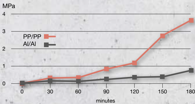
Strength development of WEICON Easy-Mix PE-PP 45 on tensile shear test samples compliant with DIN EN 1465
