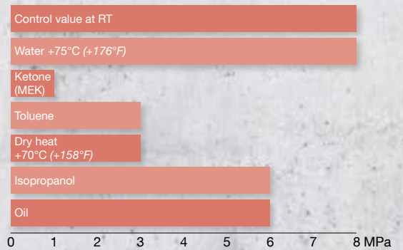
Ageing resistance of PP adhesive bonds after storage in various media (14 days at room temperature)
